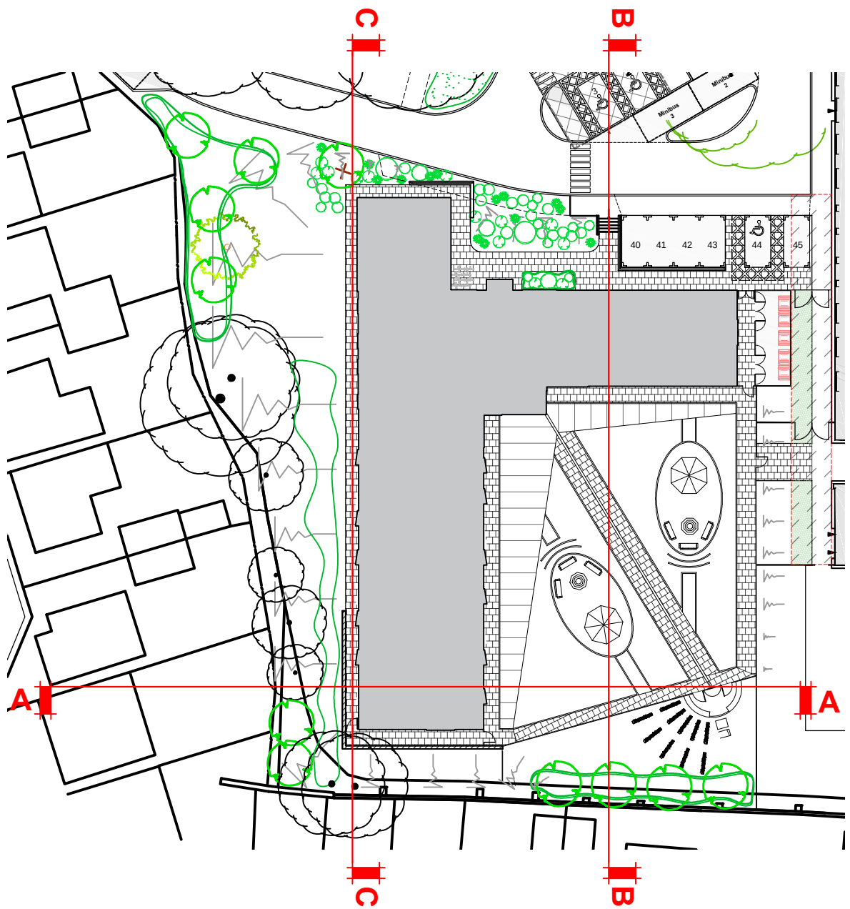
SECTION LOCATION PLAN SCALE - 1:500 @ A1
