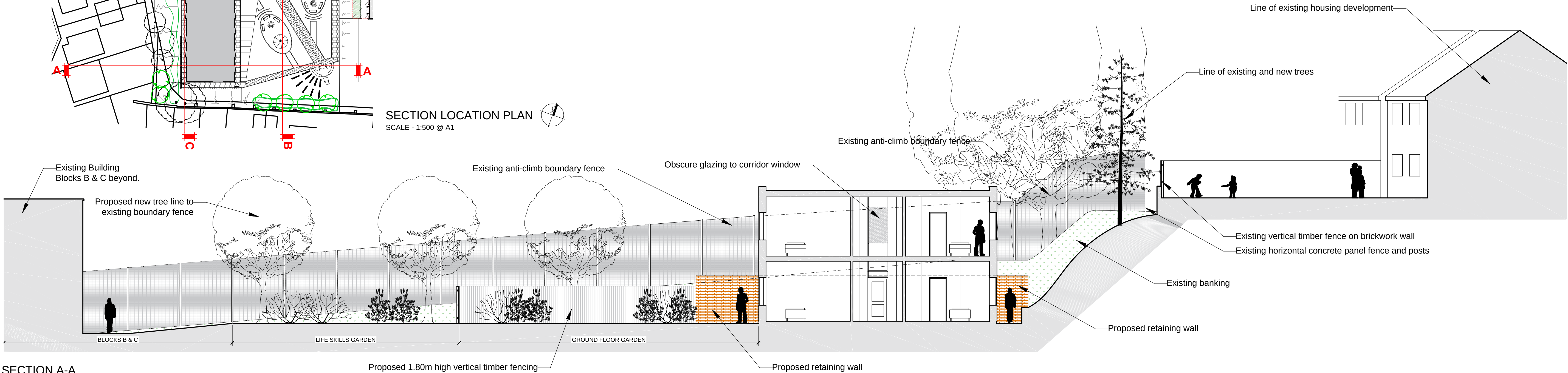
SECTION A-A SCALE - 1:100 @ A1
