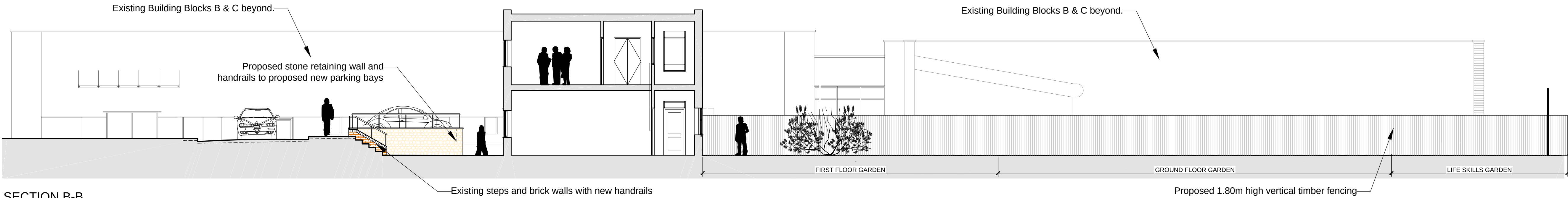
SECTION B-B SCALE - 1:100 @ A1
