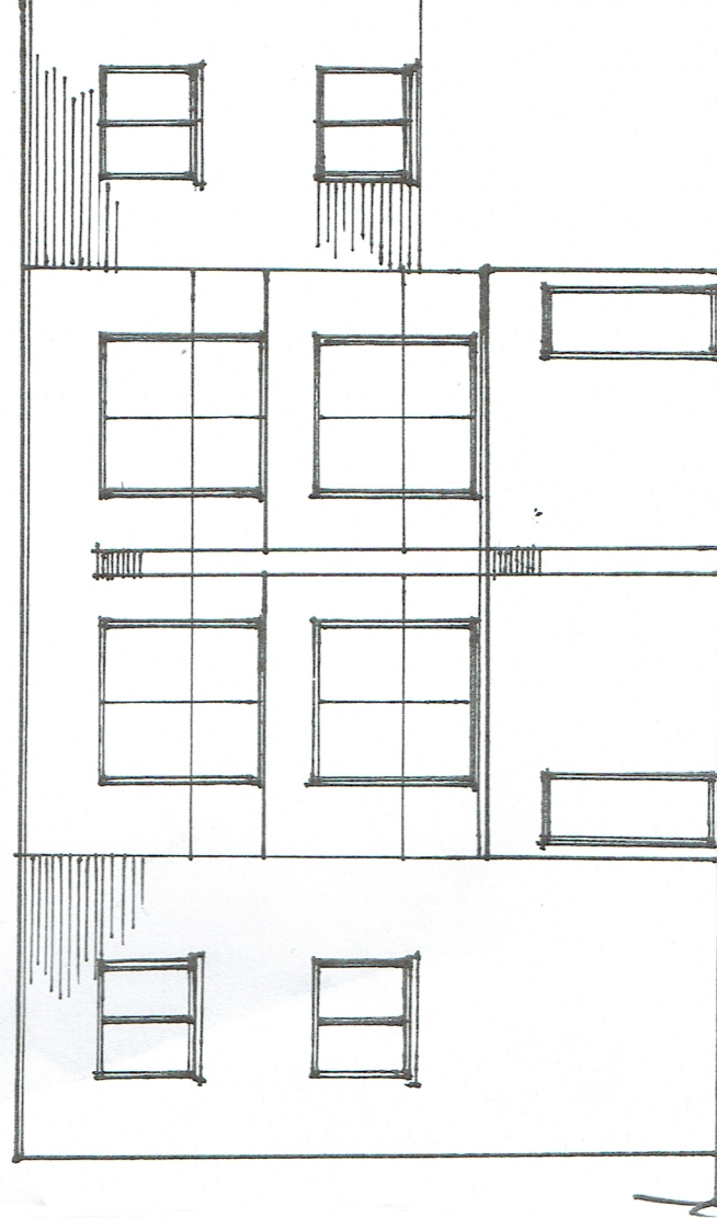
REAR ELEVATION - to CHESHAM ROAD
