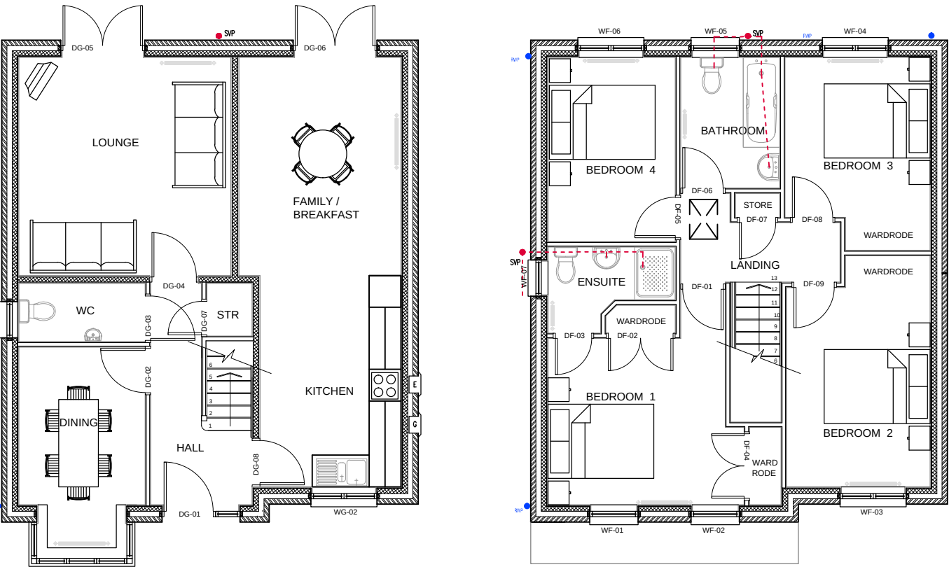
GROUND FLOOR PLAN FIRST FLOOR PLAN
