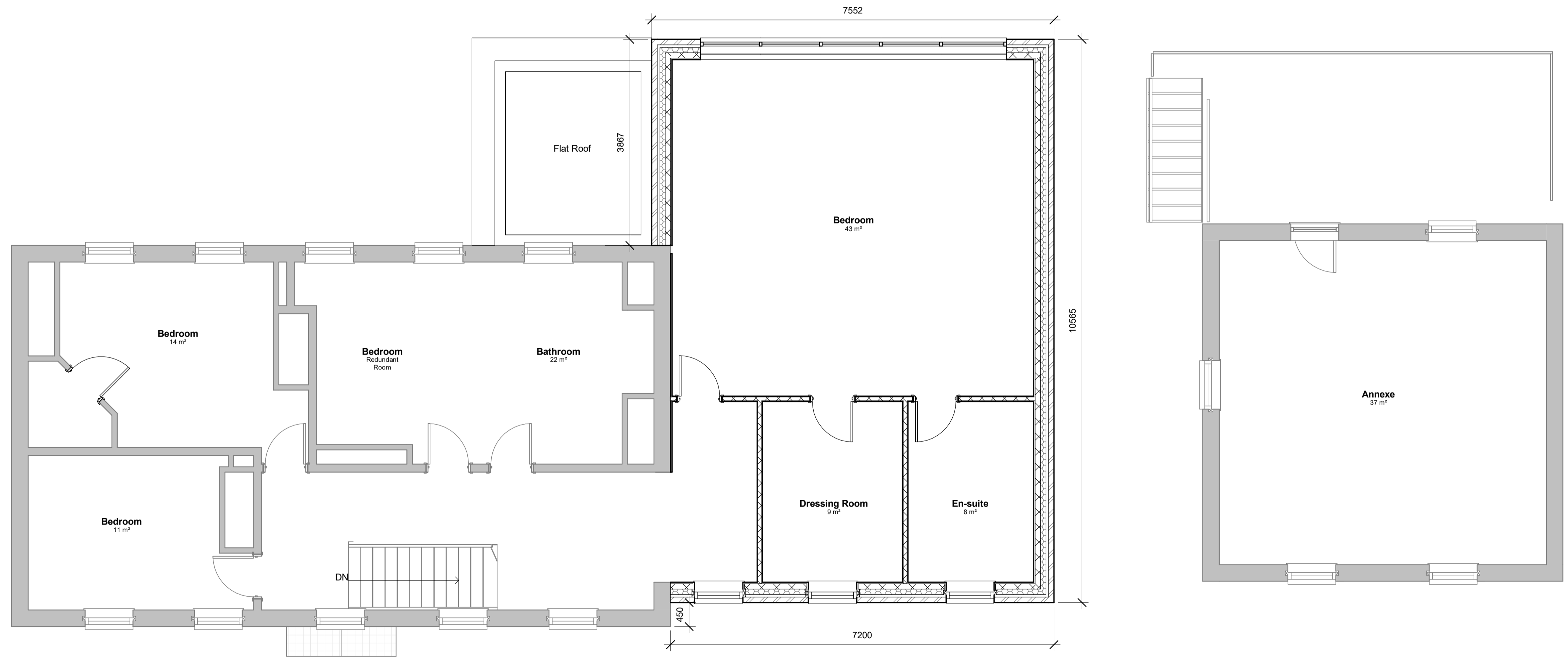
1 Proposed First Floor Plan 1 : 50
