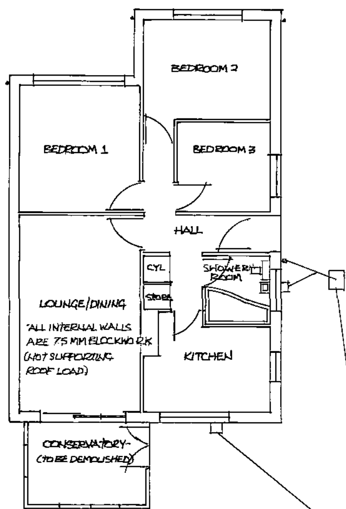
PLAN
