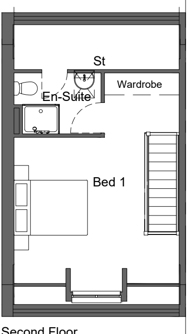
Second Floor. 1:100
