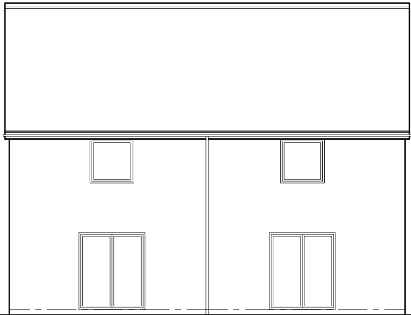
Rear Elevation (opp)
