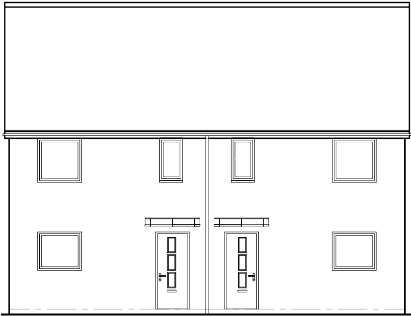
Front Elevation (as)
