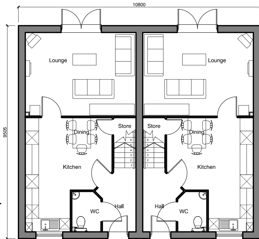
Ground Floor Plan (as)
