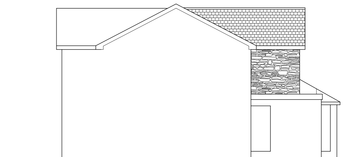
SIDE ELEVATION
