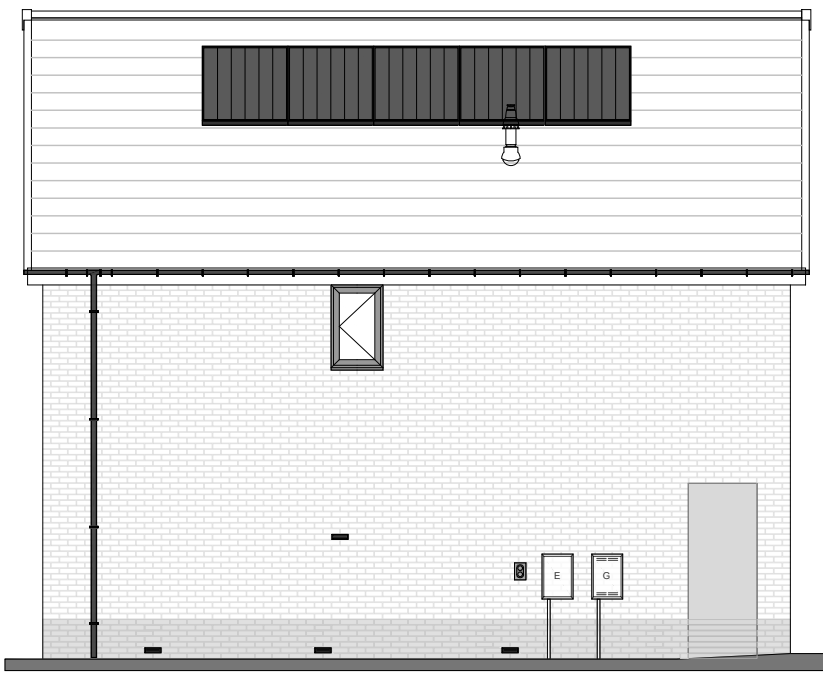
LEFT ELEVATION
