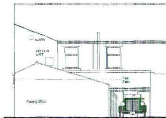
WEST (SIDE) ELEVATION (PROPOSED)
