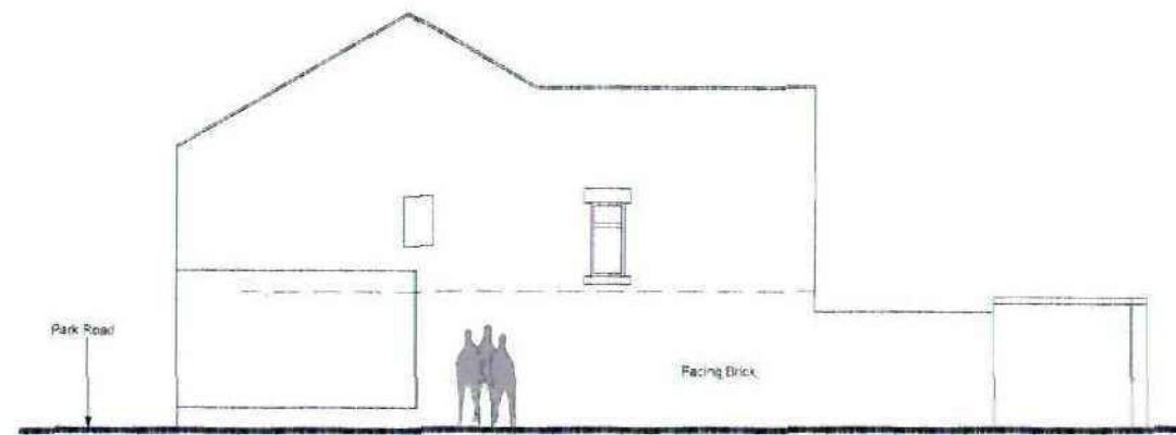
NORTH ELEVATION (EXISTING)
