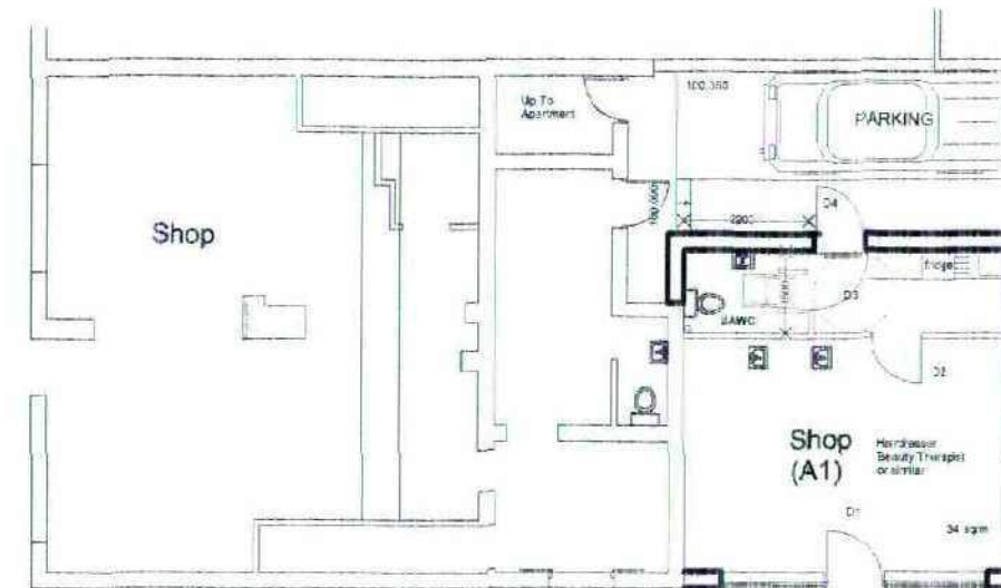
GROUND FLOOR PLAN (PROPOSED) 1:100
