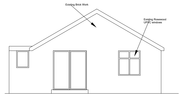
PROPOSED REAR ELEVATION (West)
