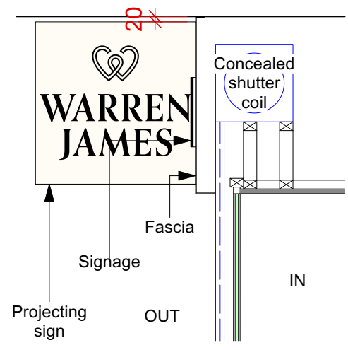
SIGN SECTION BB
