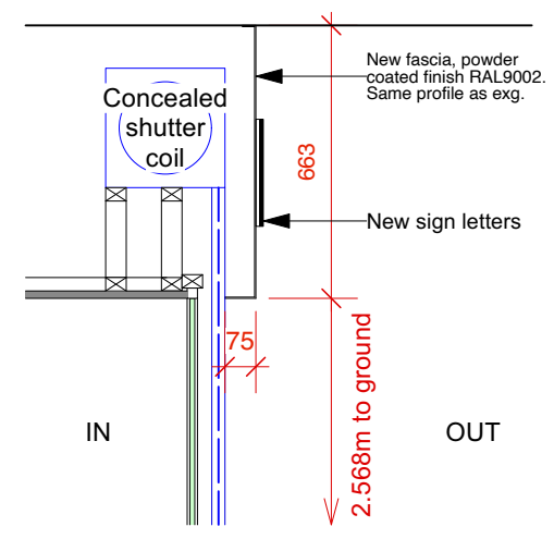
SIGN SECTION CC
