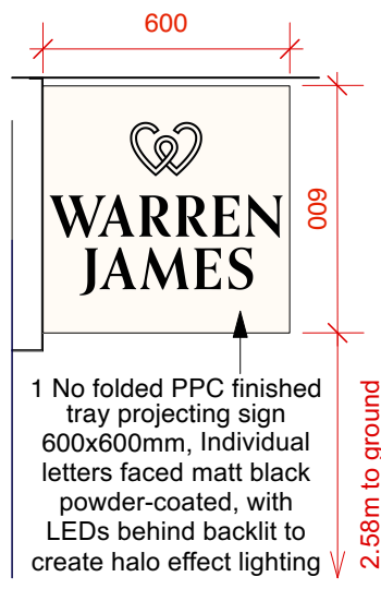
SIGN SECTION AA
