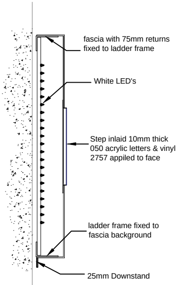
Fascia Section SCALE 1:10
