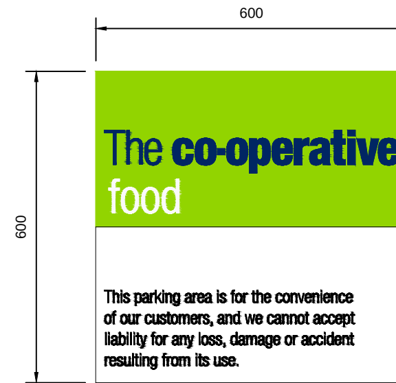
SIGN C Wall mounted Flat Panel with applied vinyl display and anti-graffitti lacquered Non illuminated SCALE 1:10
