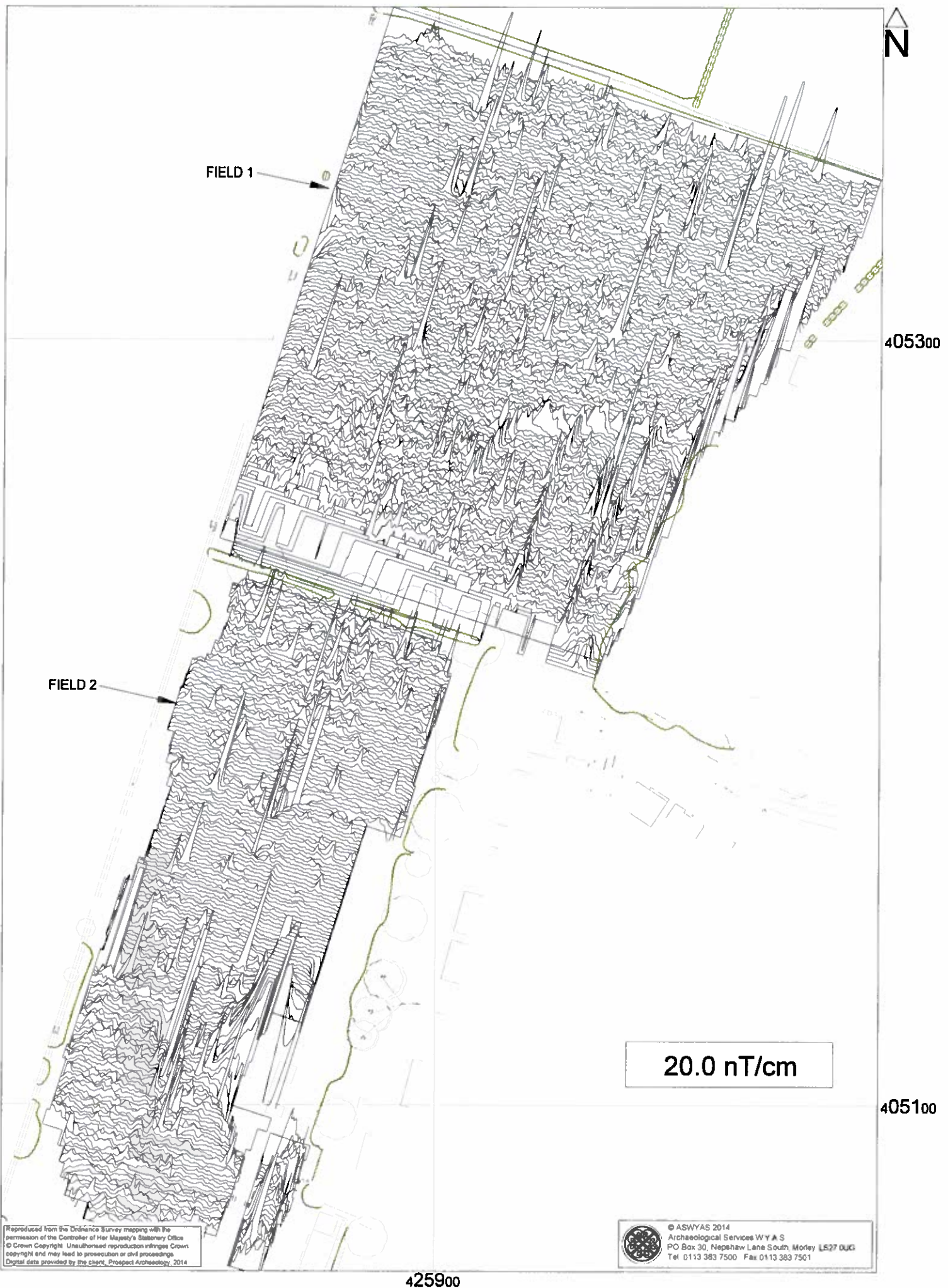
Fig. 4. XY trace plot of minimally processed magnetometer data (1:1250 @ A4) 0 40m
