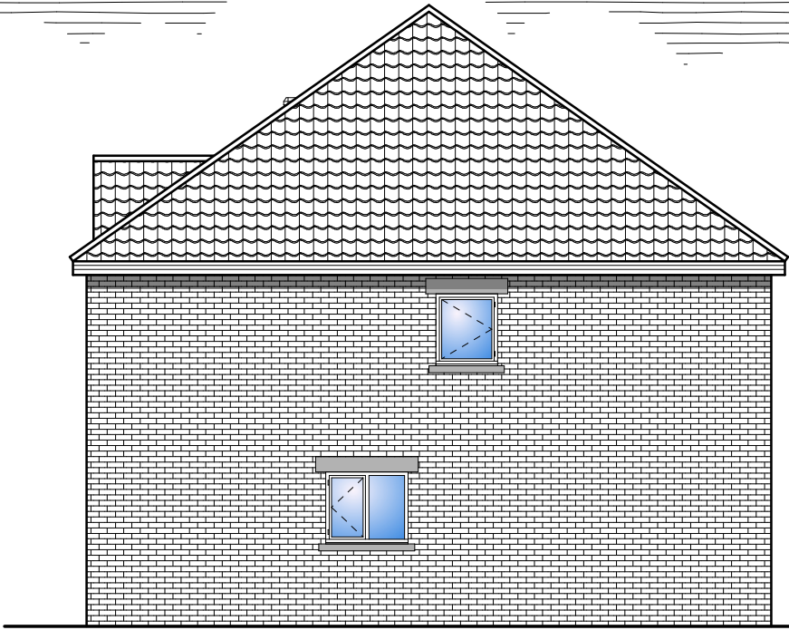
Plot 2 Side Elevation as Proposed.
