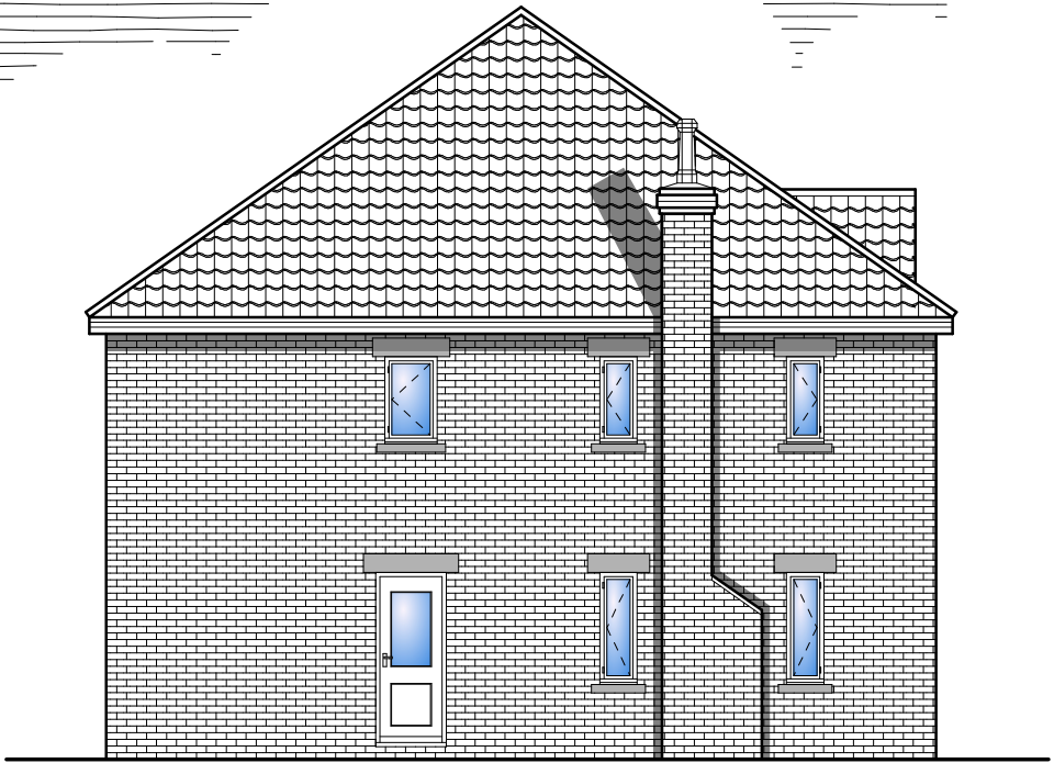
Plot 2 Side Elevation as Proposed.
