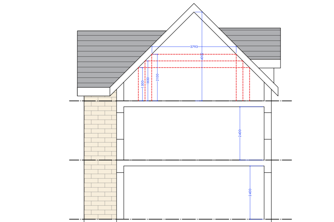
Proposed Back Elevation
