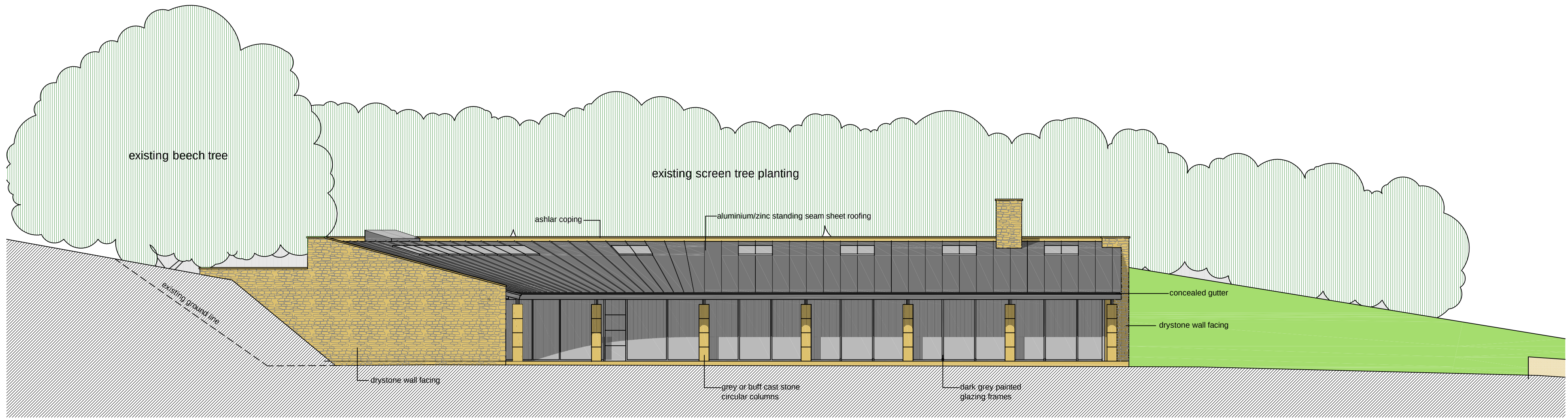
East Elevation 1:100
