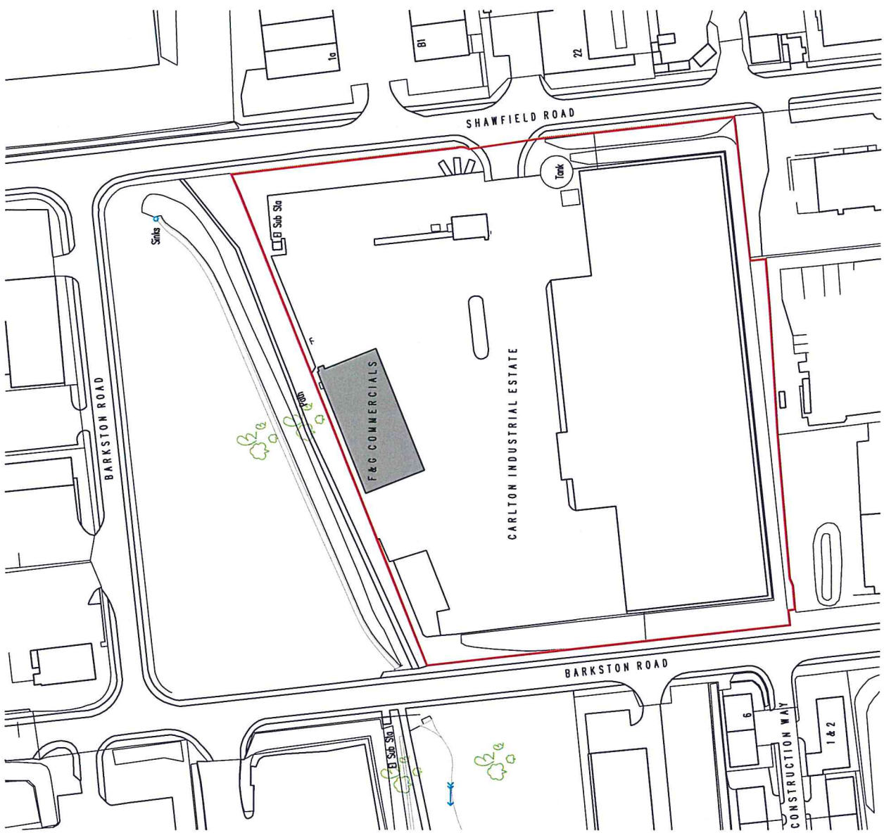
LOCATION PLAN 1:5000
