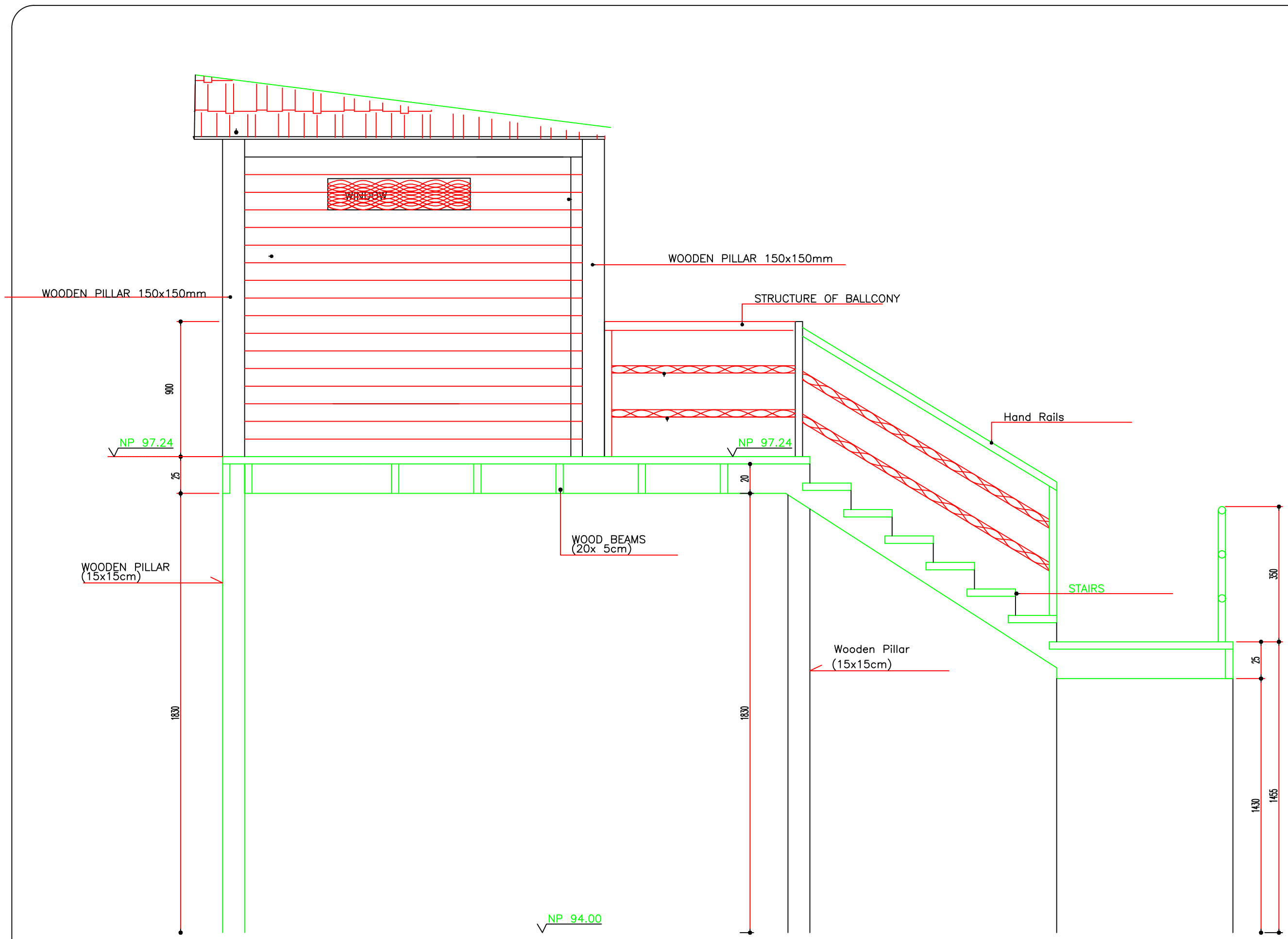
Drawing.3 – Elevation "C" – SIDE View SCALE– 1:25
