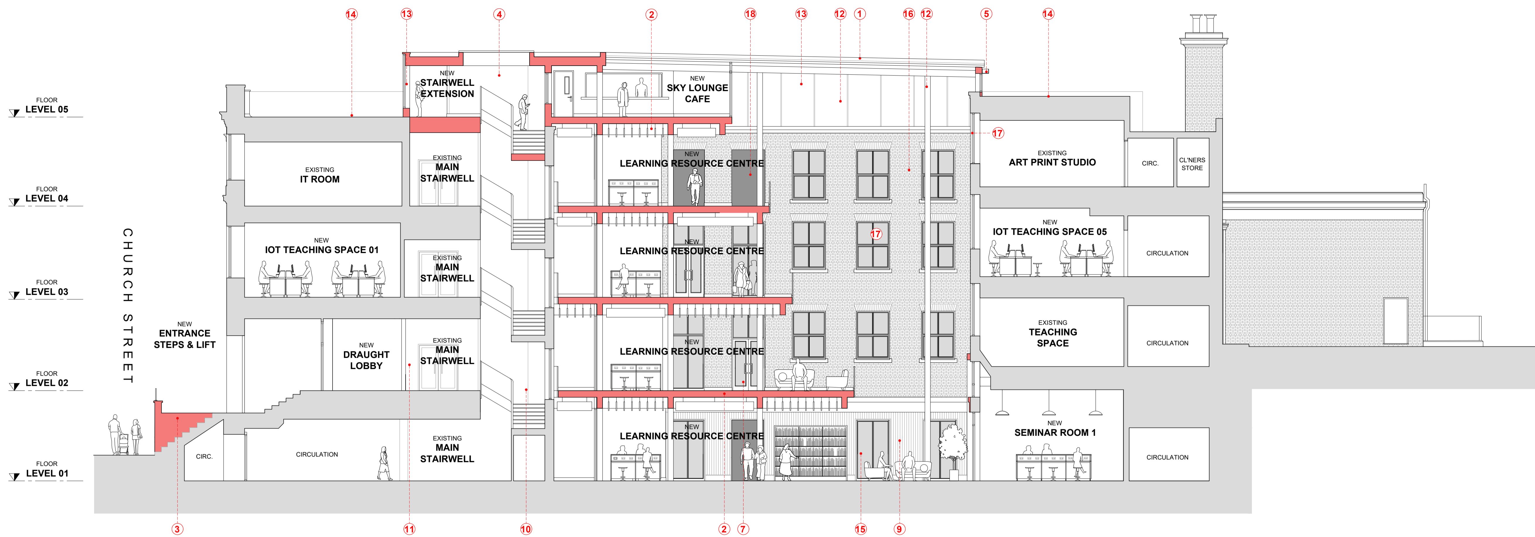
PROPOSED SECTION D-D (EAST/WEST FACING SOUTH) 1:100 @ A1
