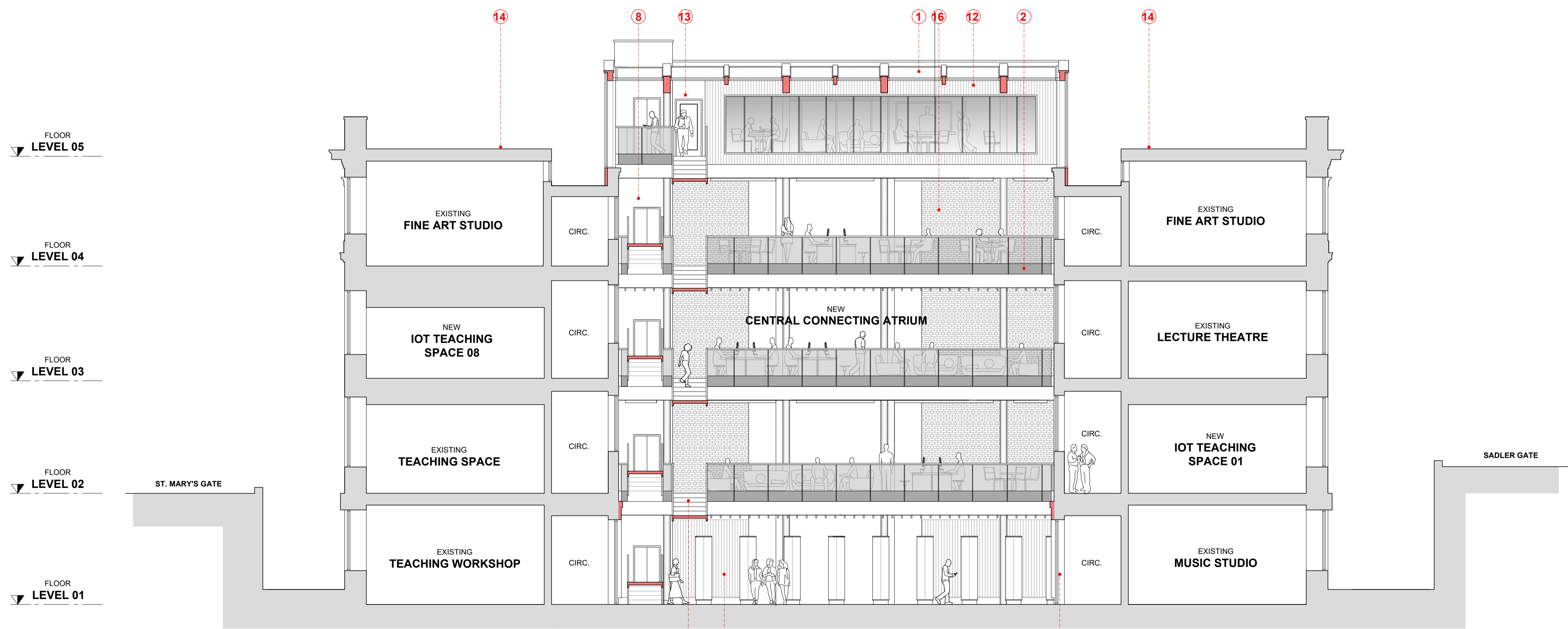
PROPOSED SECTION E-E (NORTH/SOUTH FACING EAST) 1:100 @ A1
