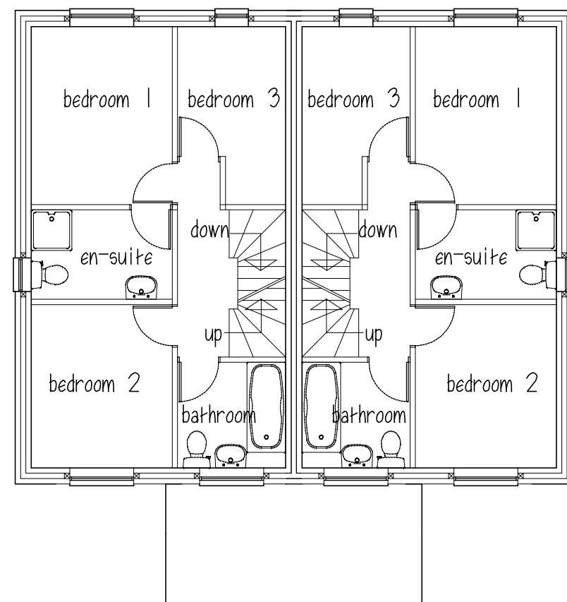
FIRST FLOOR
