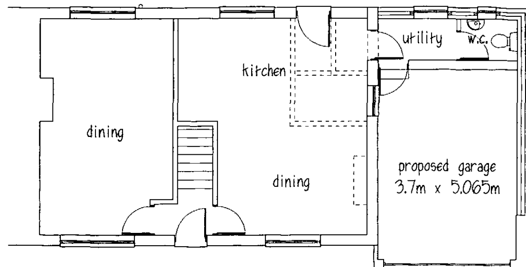
GROUND FLOOR
