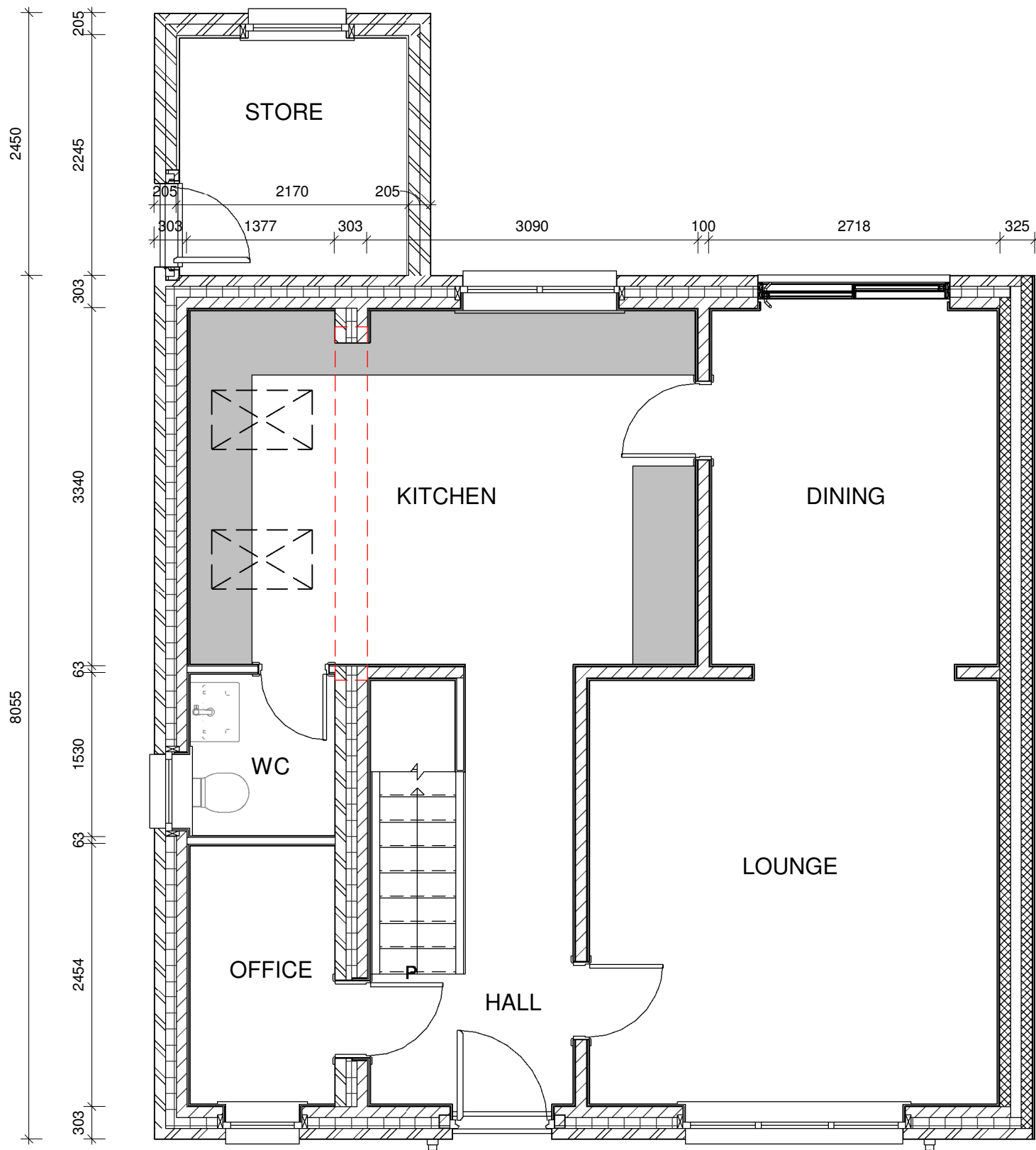
Proposed Ground Floor G.A 1 : 50
