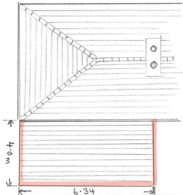
PLAN - SHOWING EXTENSION ●
