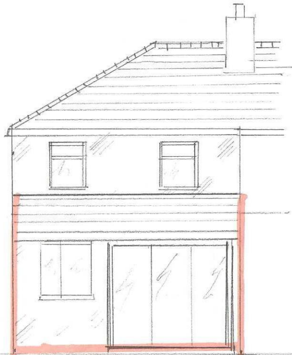
REAR ELEVATION + EXTENSION ●
