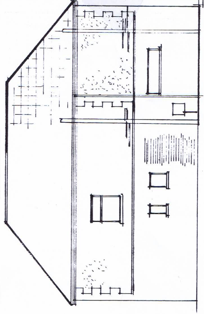
PROPOSED SIDE
