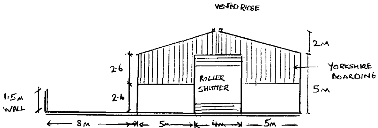
FRONT ELEVATION (REAR ELEVATION SIMILAR)
