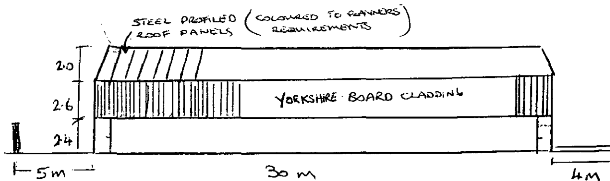
SIDE ELEVATION,
