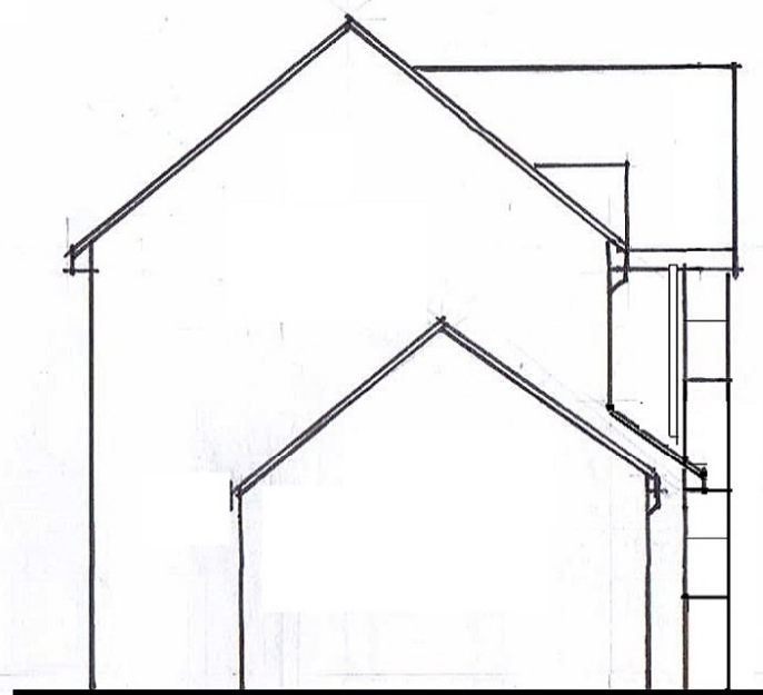
EXISTING LEFT SIDE ELEVATION
