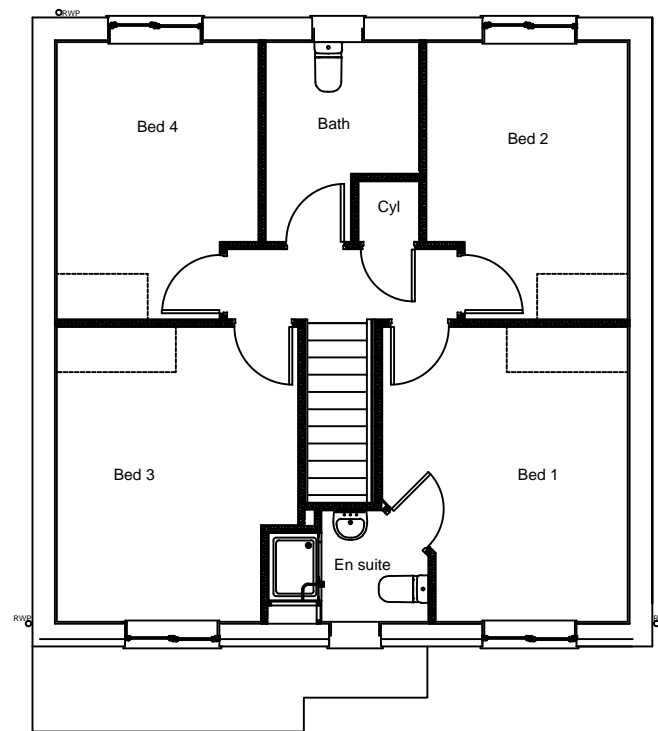
Baybridge Brick FIRST FLOOR PLAN
