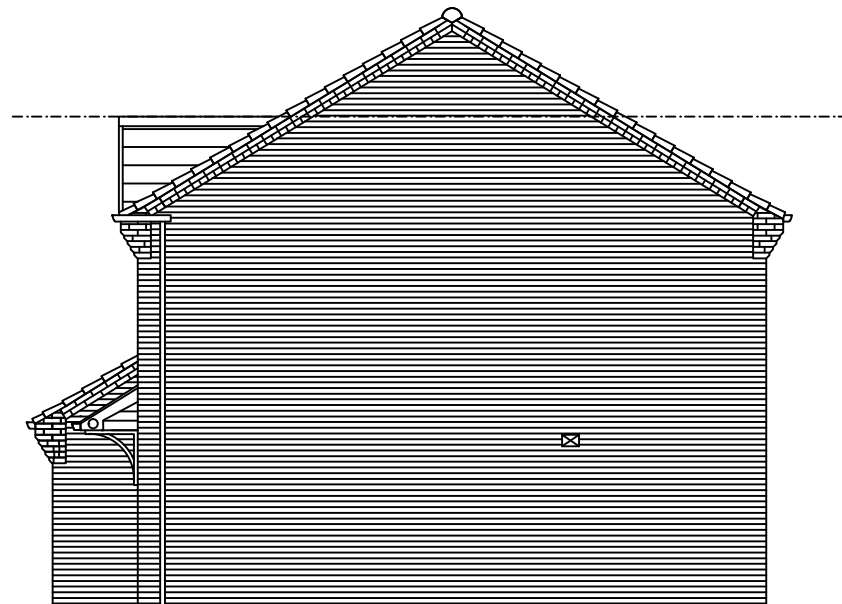
Baybridge Brick SIDE ELEVATION
