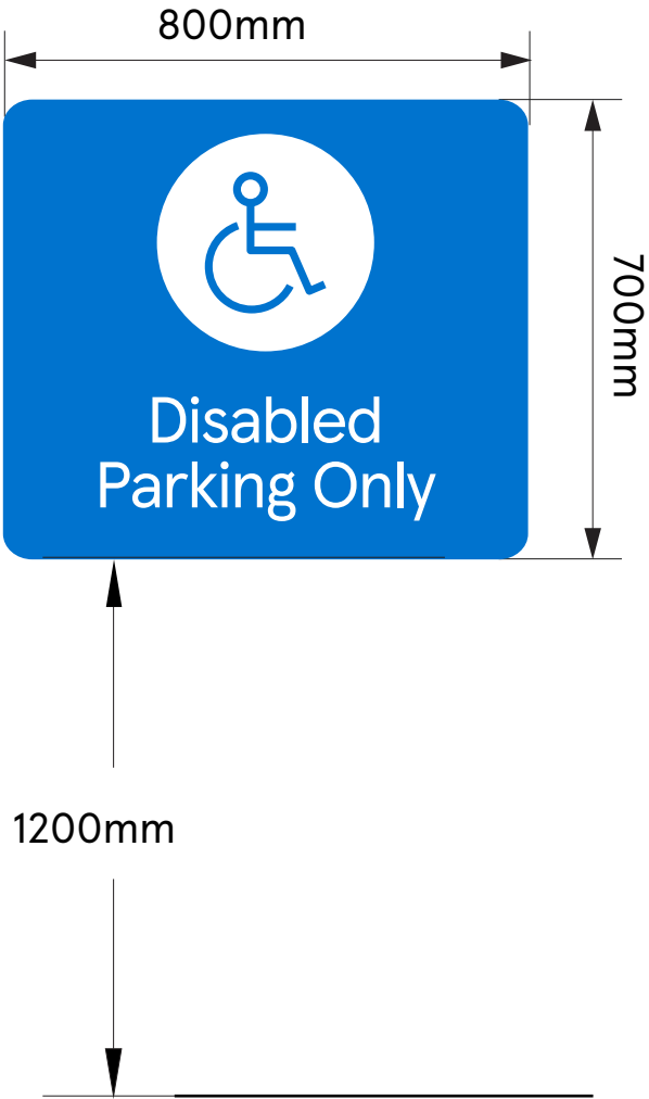
New Wall mounted Disabled Car Park Sign Inset Scale - 1 : 20
