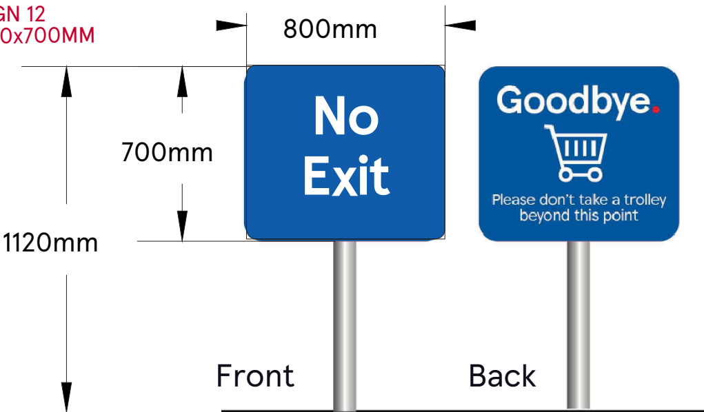
Pole mounted No Exist / Goodbye signs SIZE : 800X1120mm Inset Scale - 1 : 20
