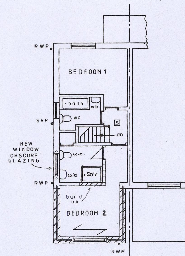
PROPOSED F.F. PLAN
