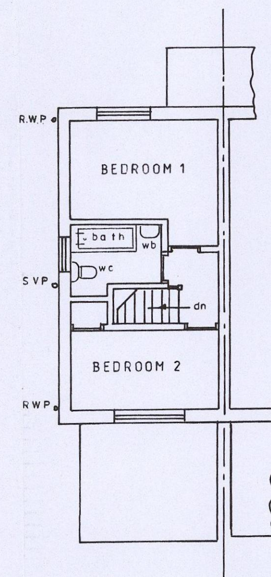
EXISTING F.F. PLAN
