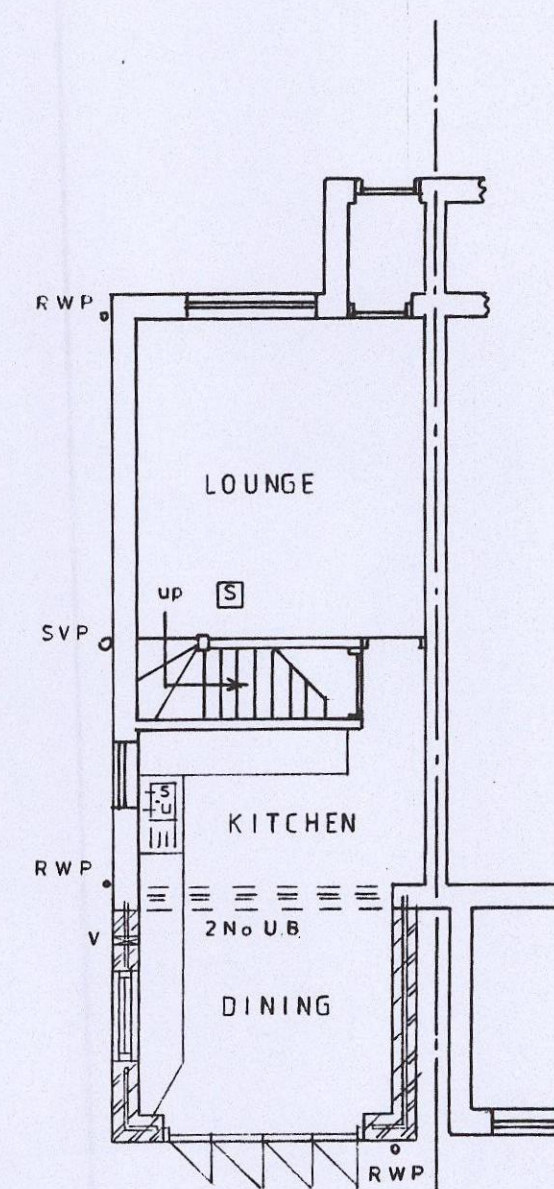
PROPOSED G.F. PLAN
