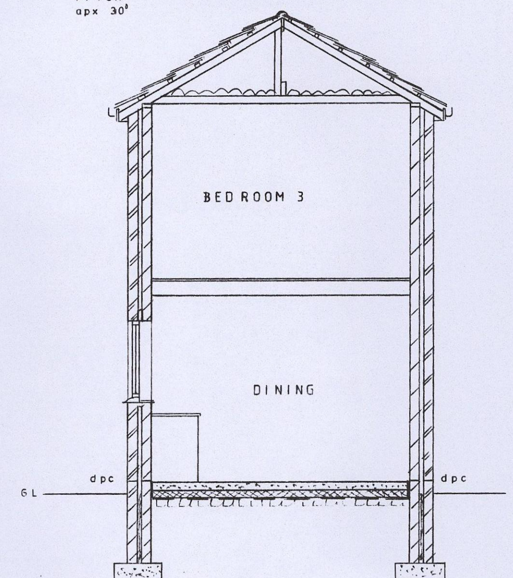
SECTION 1:50
