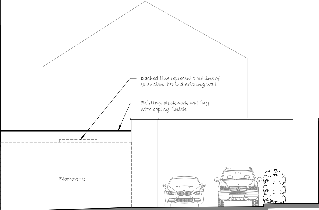
PROPOSED WEST ELEVATION (VIEW FROM CAR PARK AREA) SCALE - 1:100
