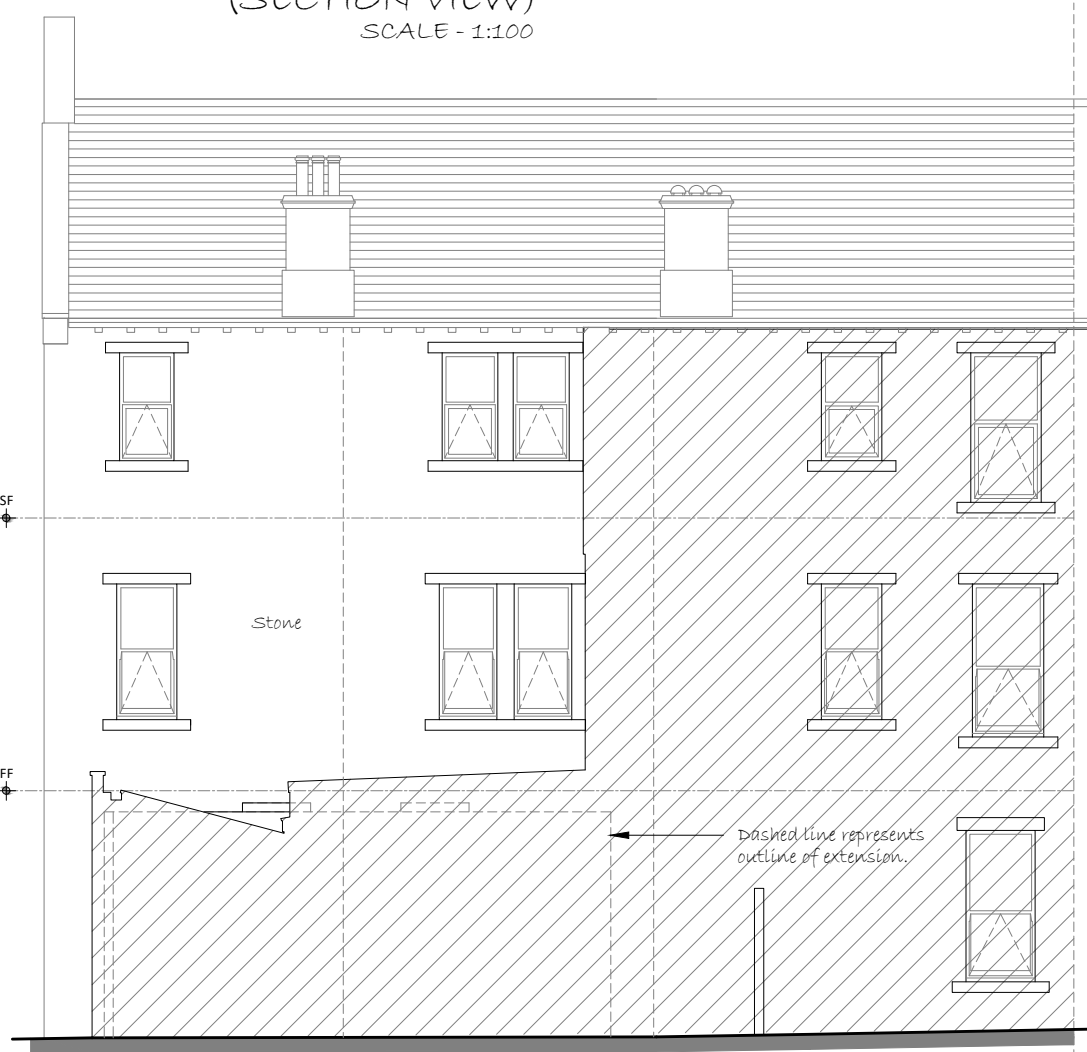
PROPOSED SOUTH ELEVATION SCALE - 1:100
