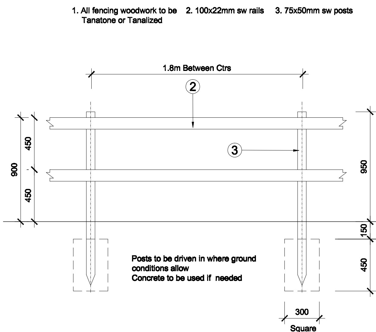
900mm High Post & Rail Fence (7)
