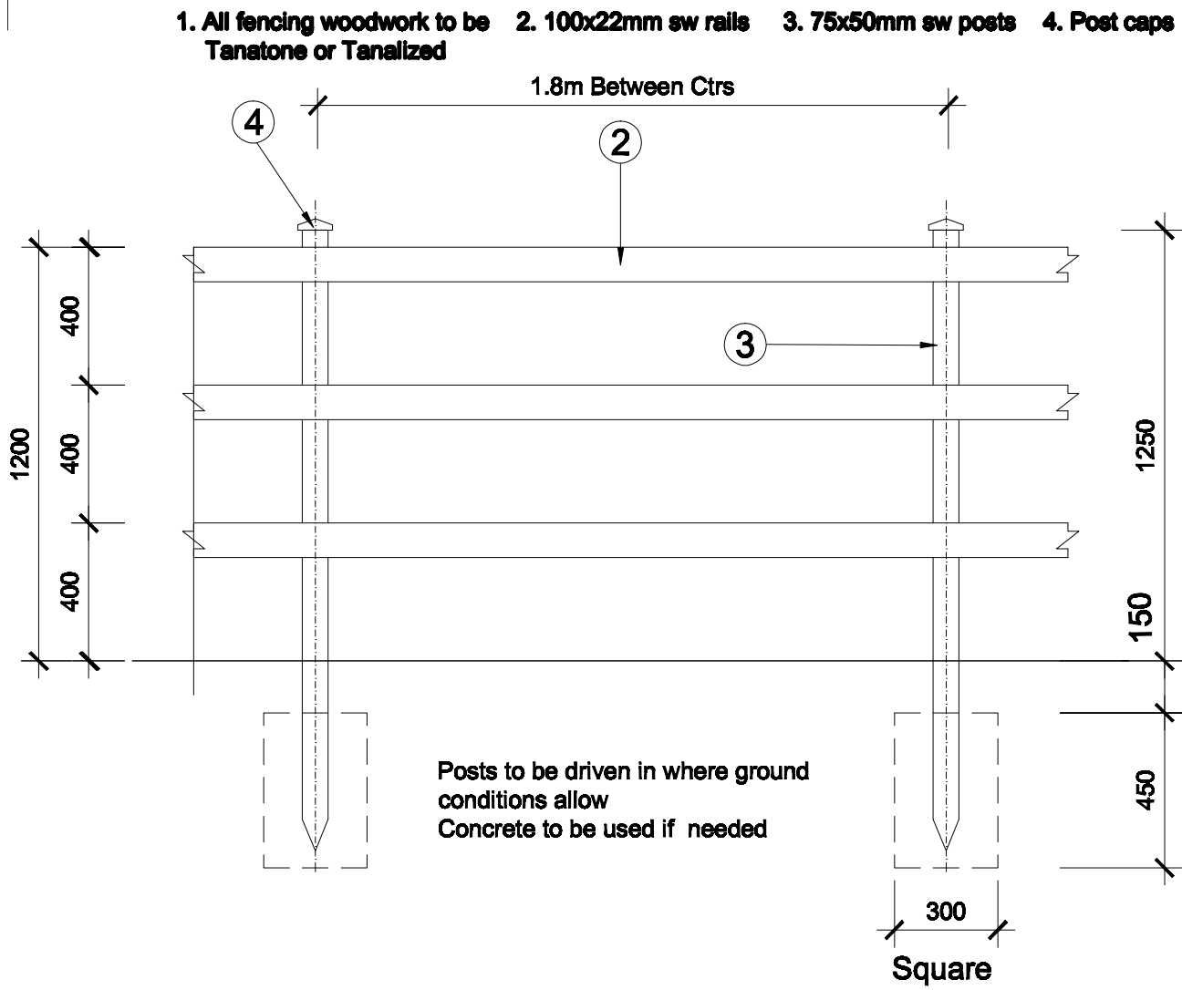
1200mm High Post and Rail Fence (10)
