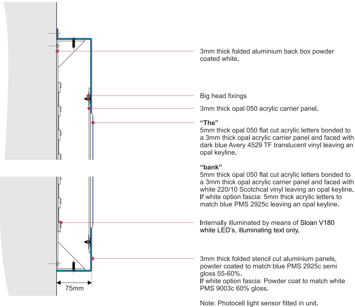
Section through "The" and "bank" - scale 1:5 @ A3
