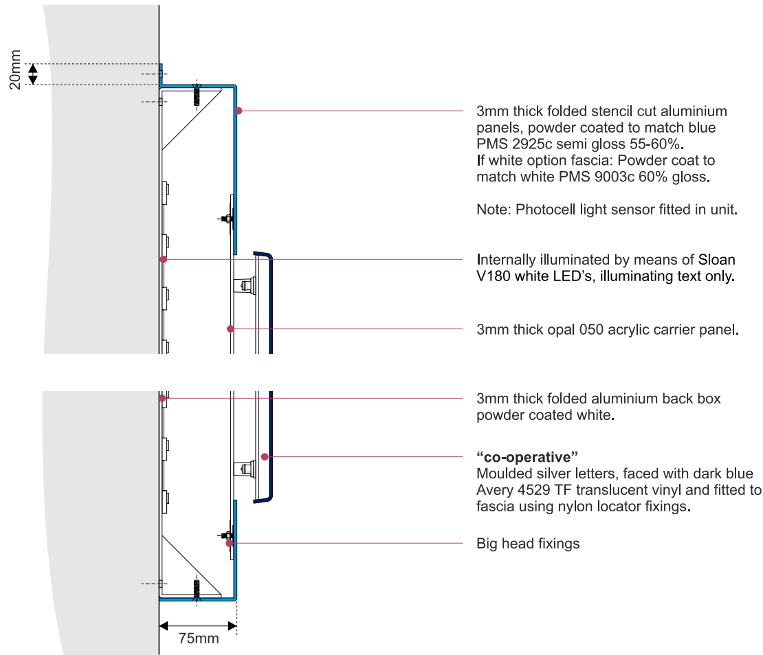
Section through "co-operative" - scale 1:5 @ A3
