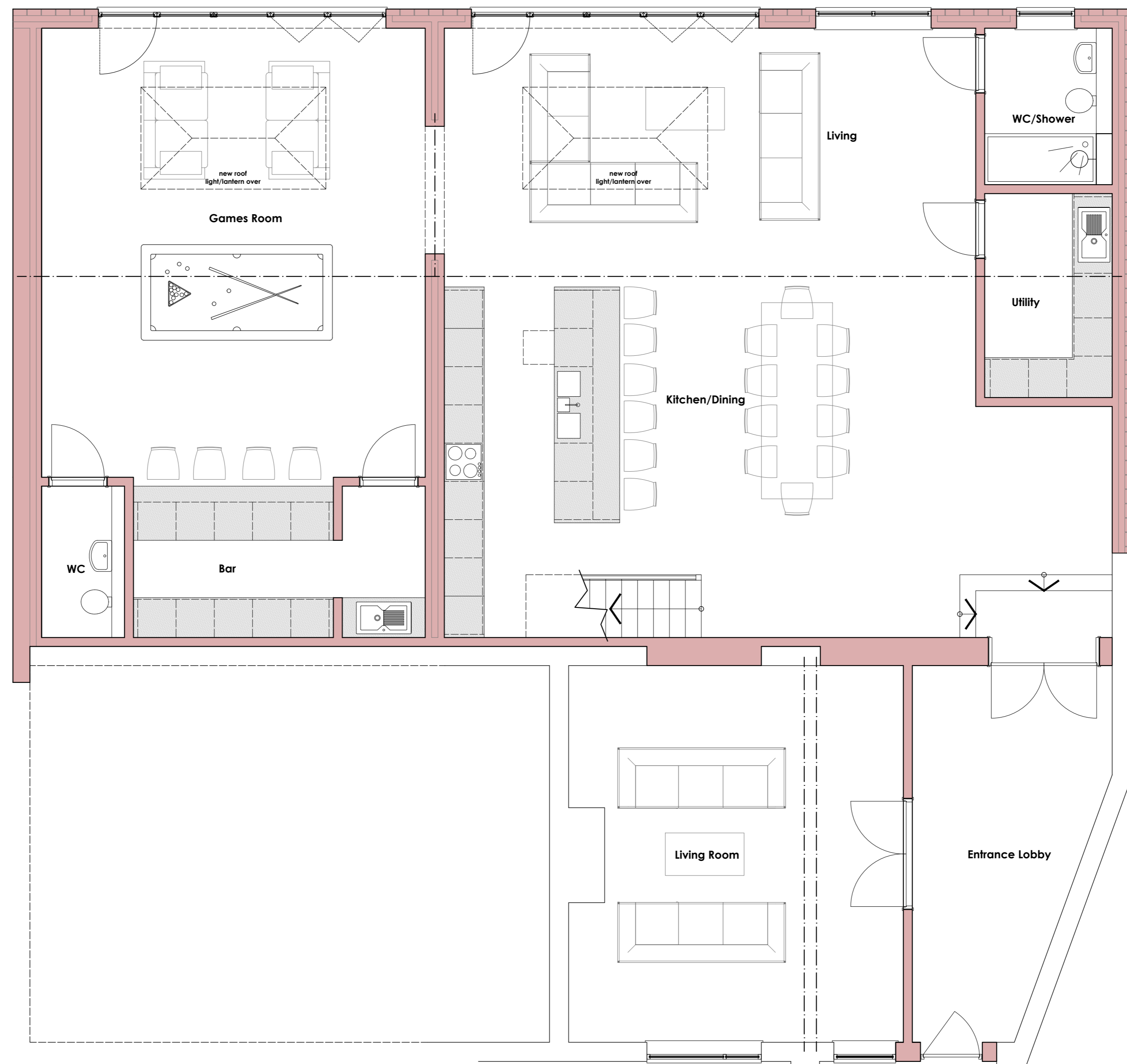
— New walls - - - New structure to be designed by Structural Engineer FIRST FLOOR - as proposed Scale 1:50 @ A1
