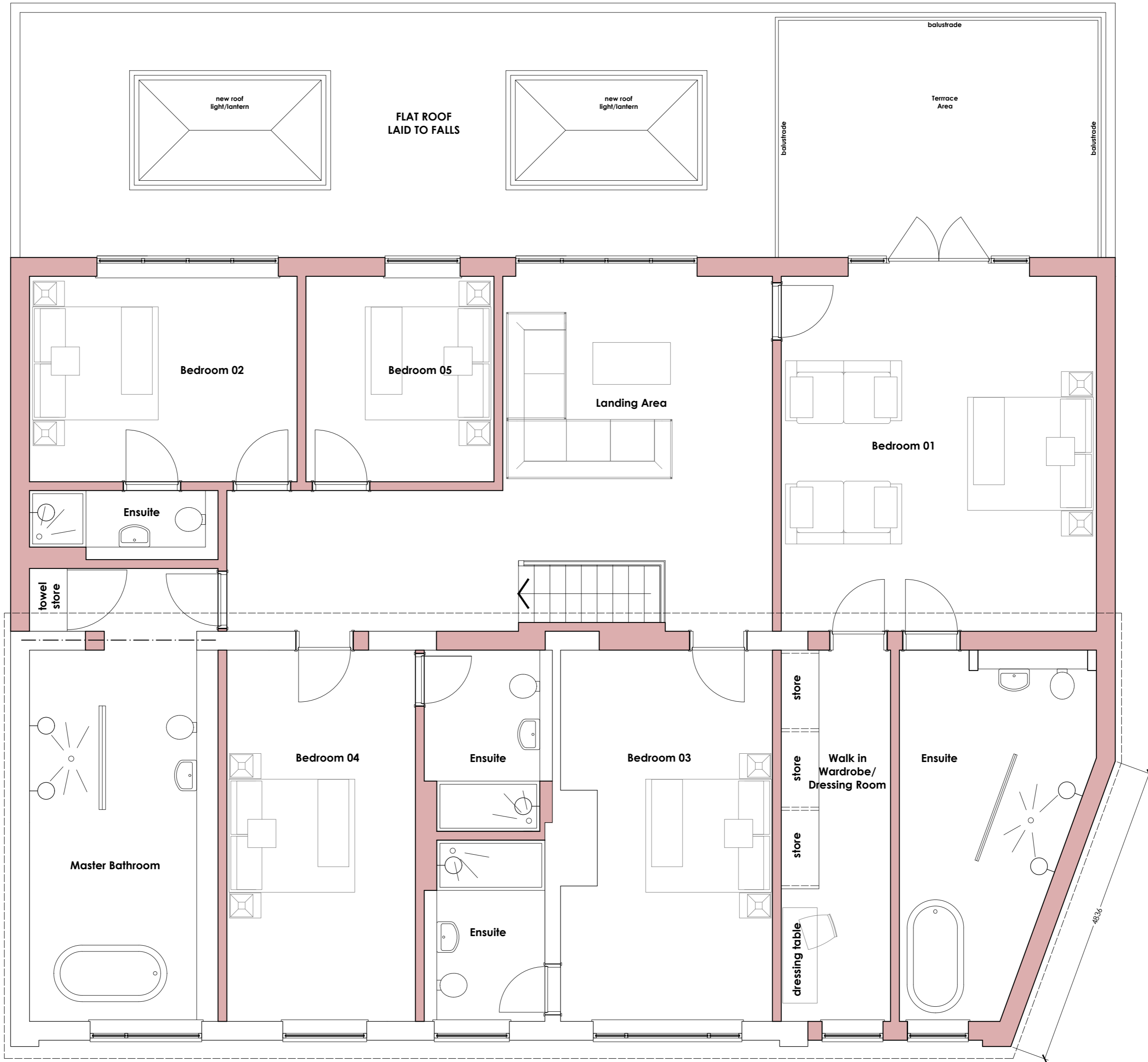
— New walls - - - New structure to be designed by Structural Engineer GROUND FLOOR - as proposed Scale 1:50 @ A1
