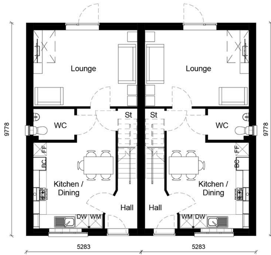
Ground Floor. 1 : 100
