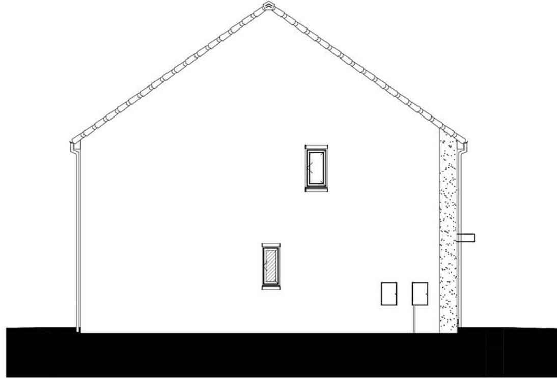
Left Elevation. 1 : 100
