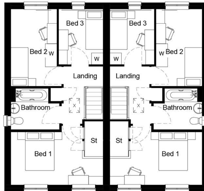
First Floor. 1 : 100
