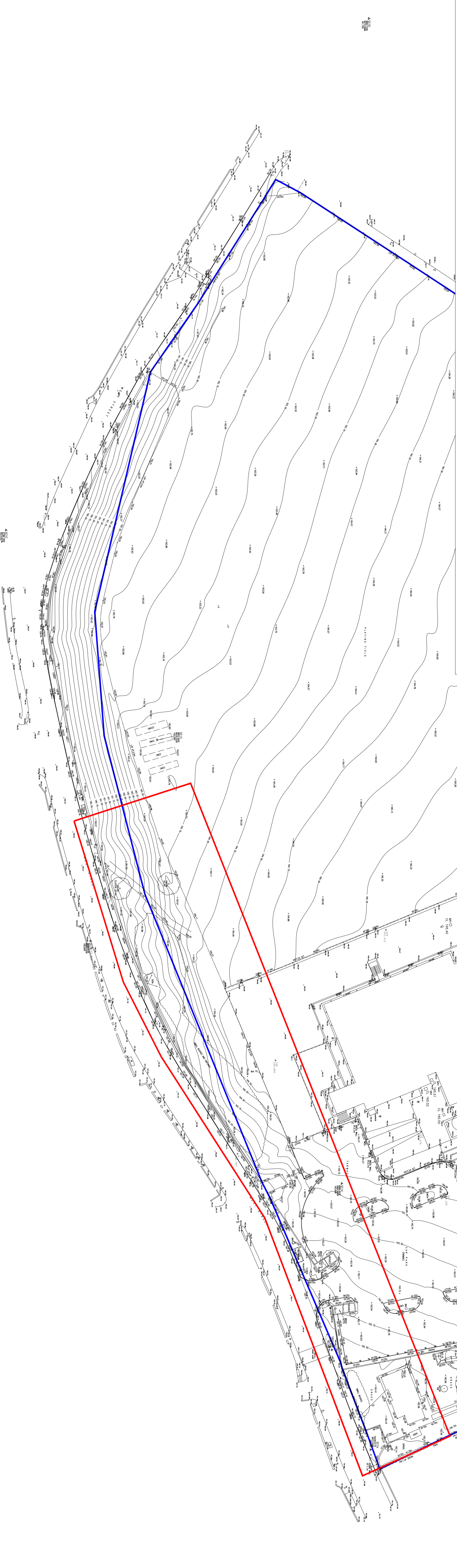
Full Site Topographical Survey - 1:2000
