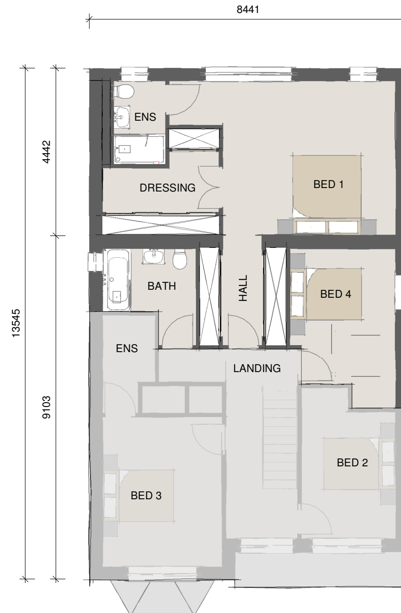
First Floor. 1 : 100
