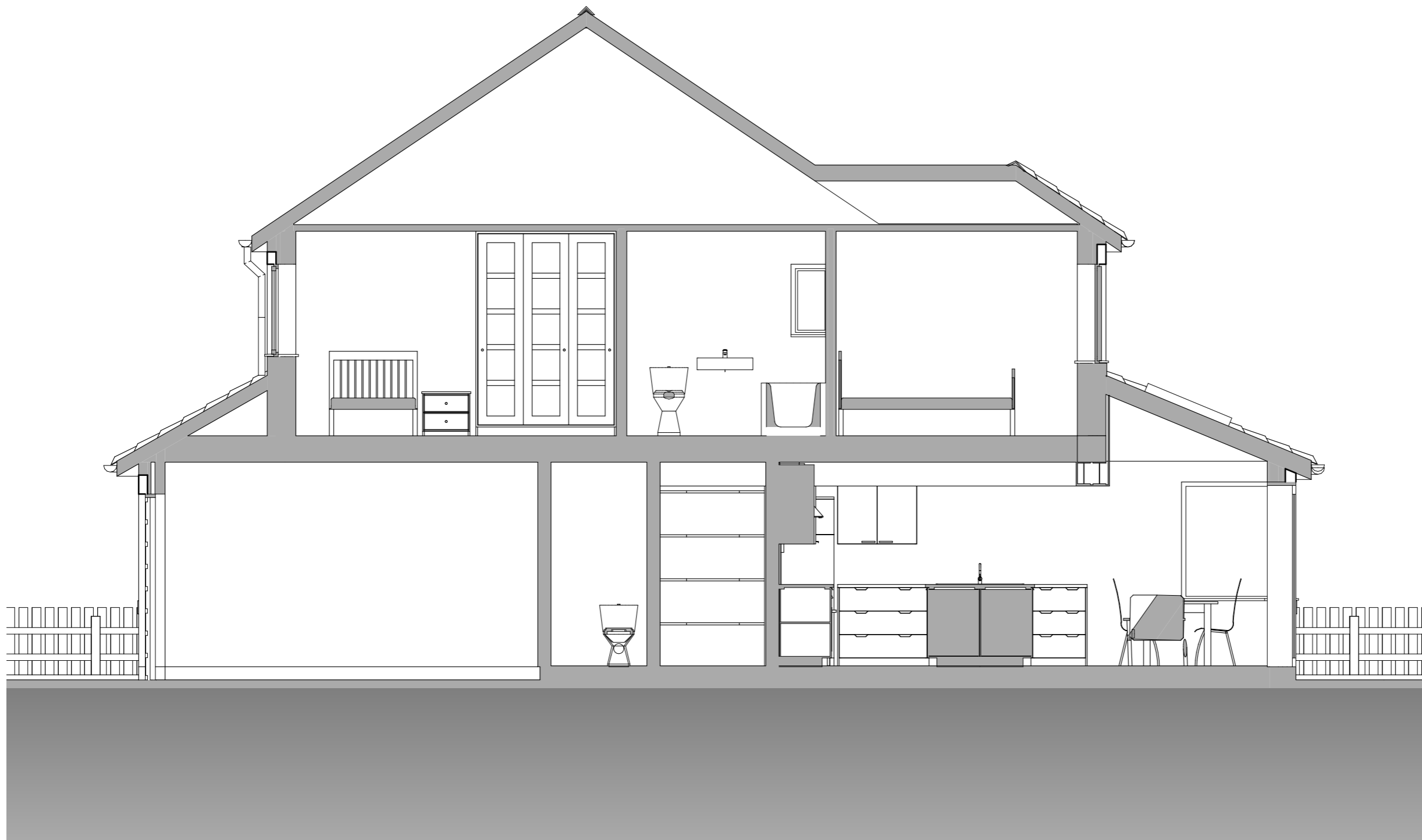
Building Section A-A
