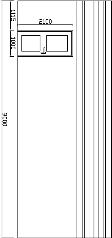
Side Elevation
