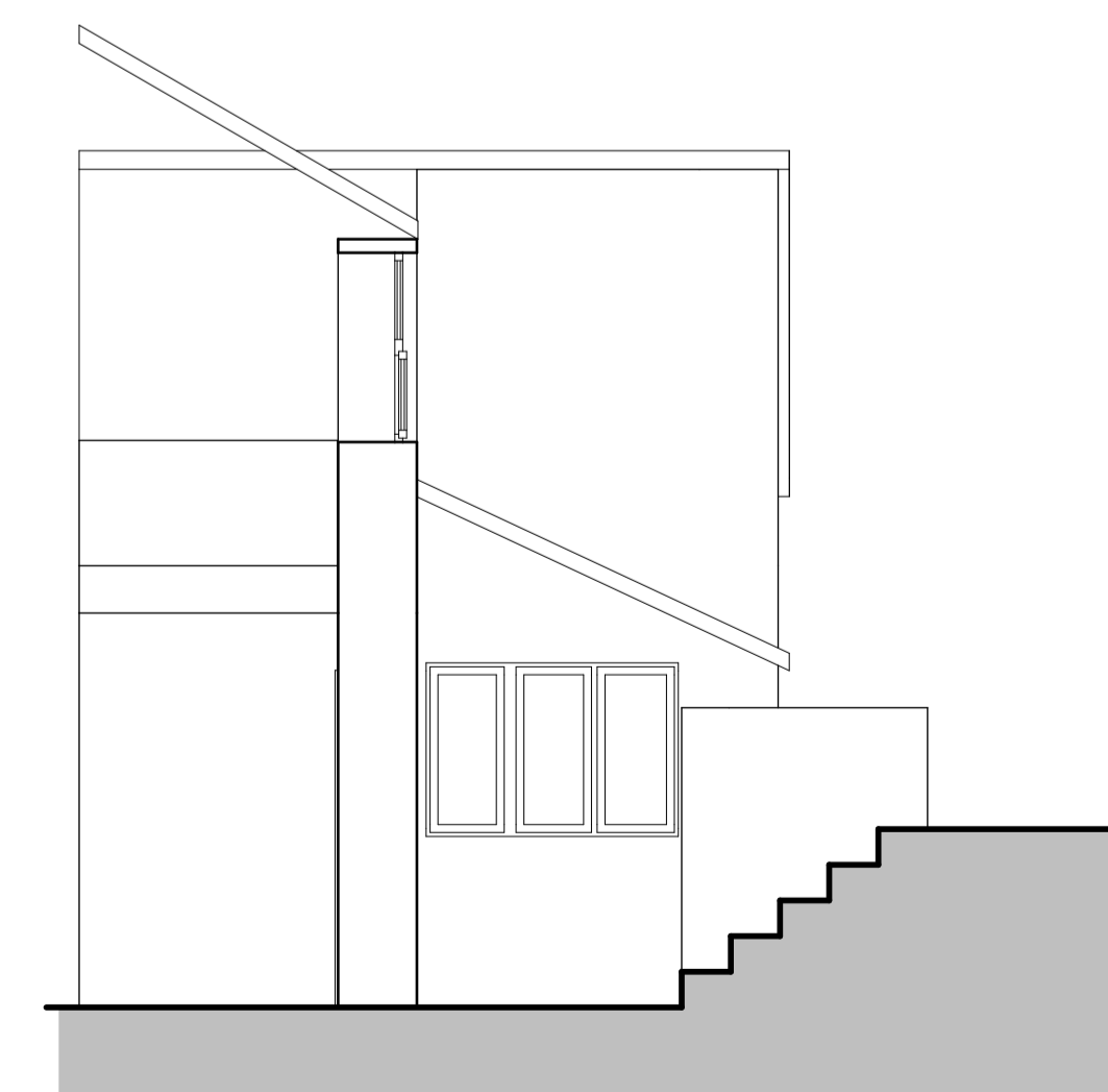
S-49 Building Section 1:50
