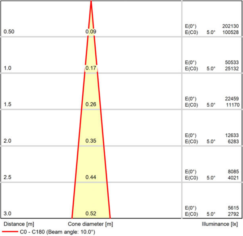
Cone diagram
