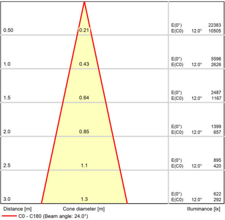
Cone diagram
