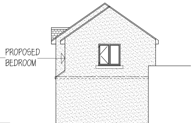
SIDE ELEVATION
