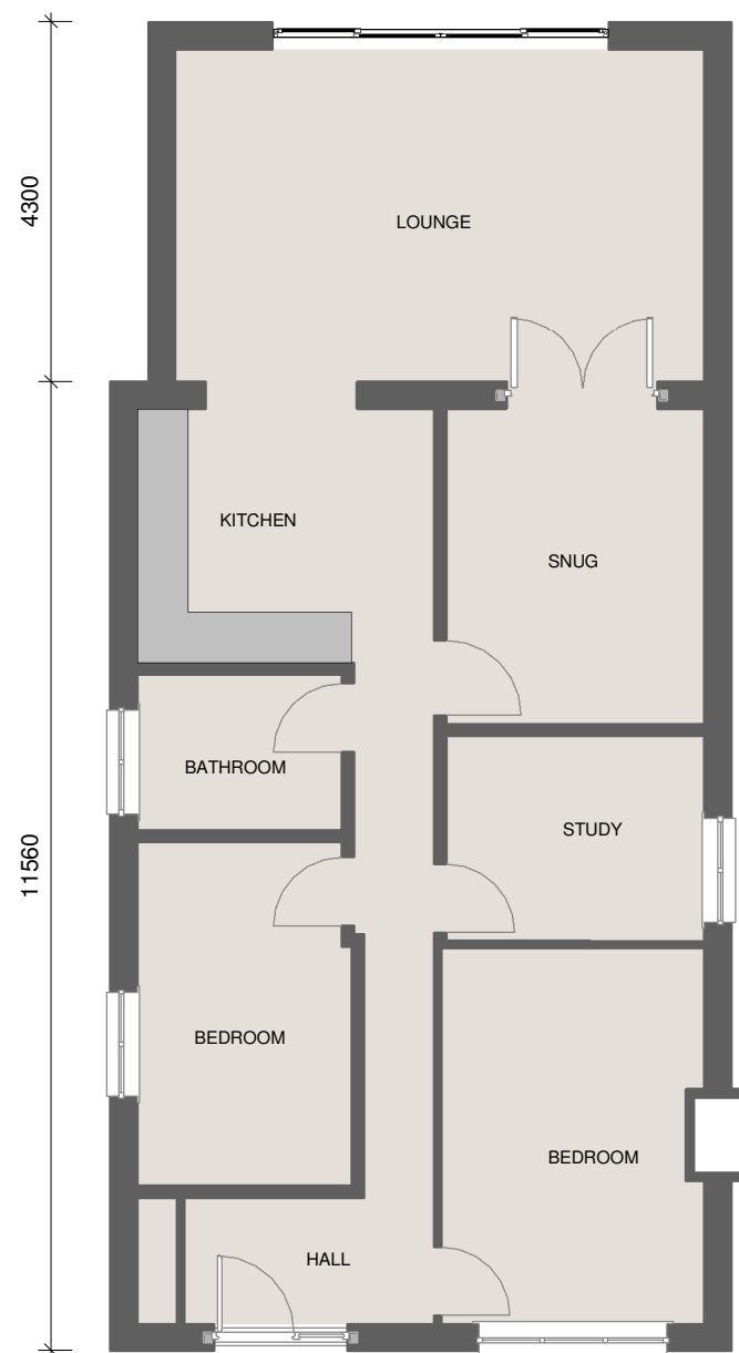
Ground Floor 1 : 100
