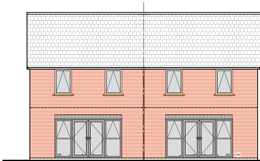
Rear Elevation
