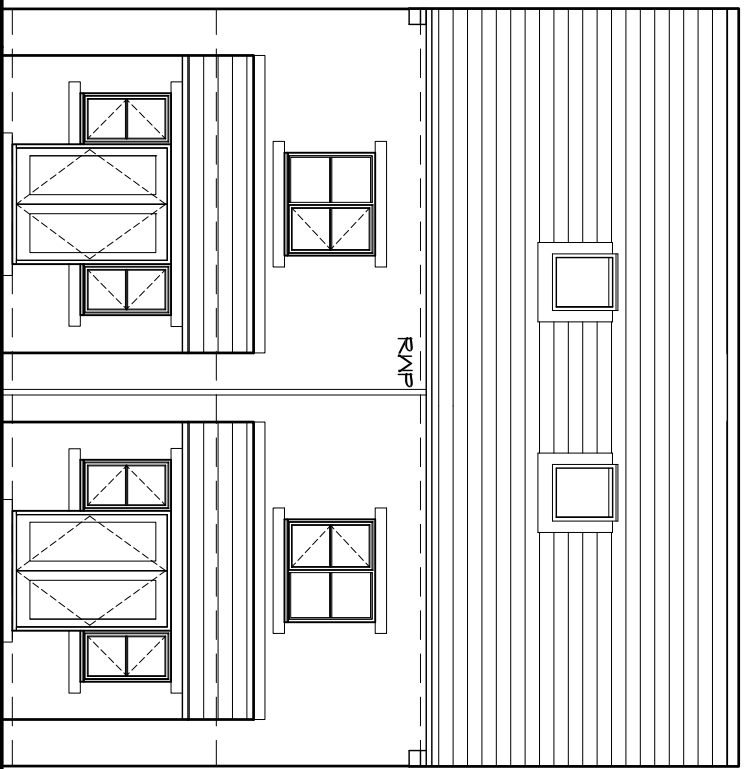
Rear Elevation Scale 1:100
