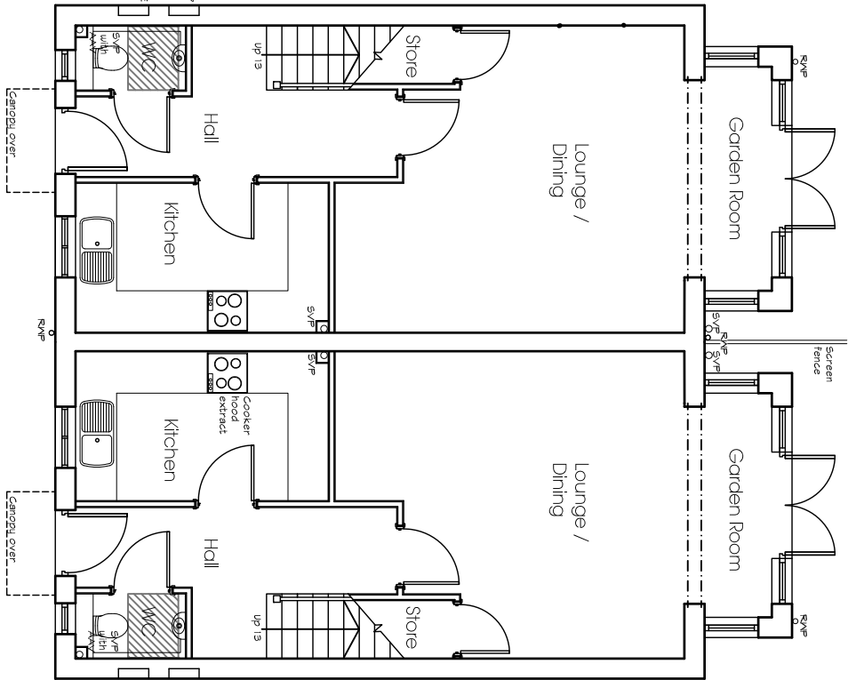
Ground Floor Scale - 1:50
