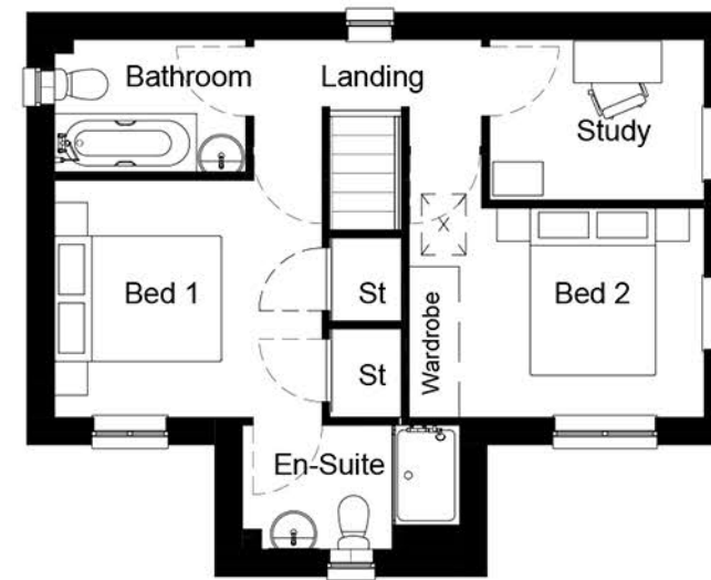
First Floor. 1 : 100
