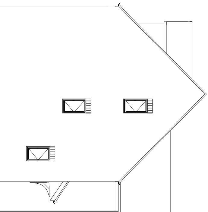
Side Elevation
