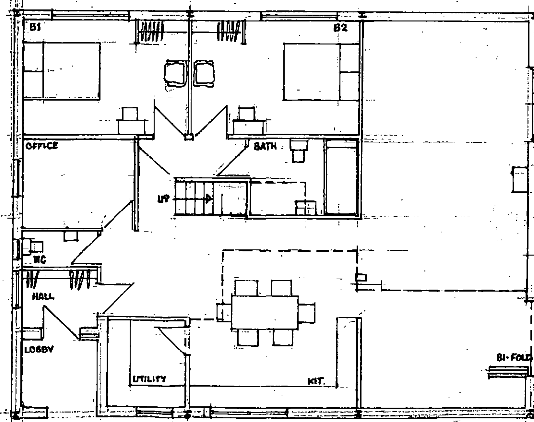
BARN CONVERSION - UPPER BELL CLIVE FARM PLANS 1:100 DRG A1 3/2020
