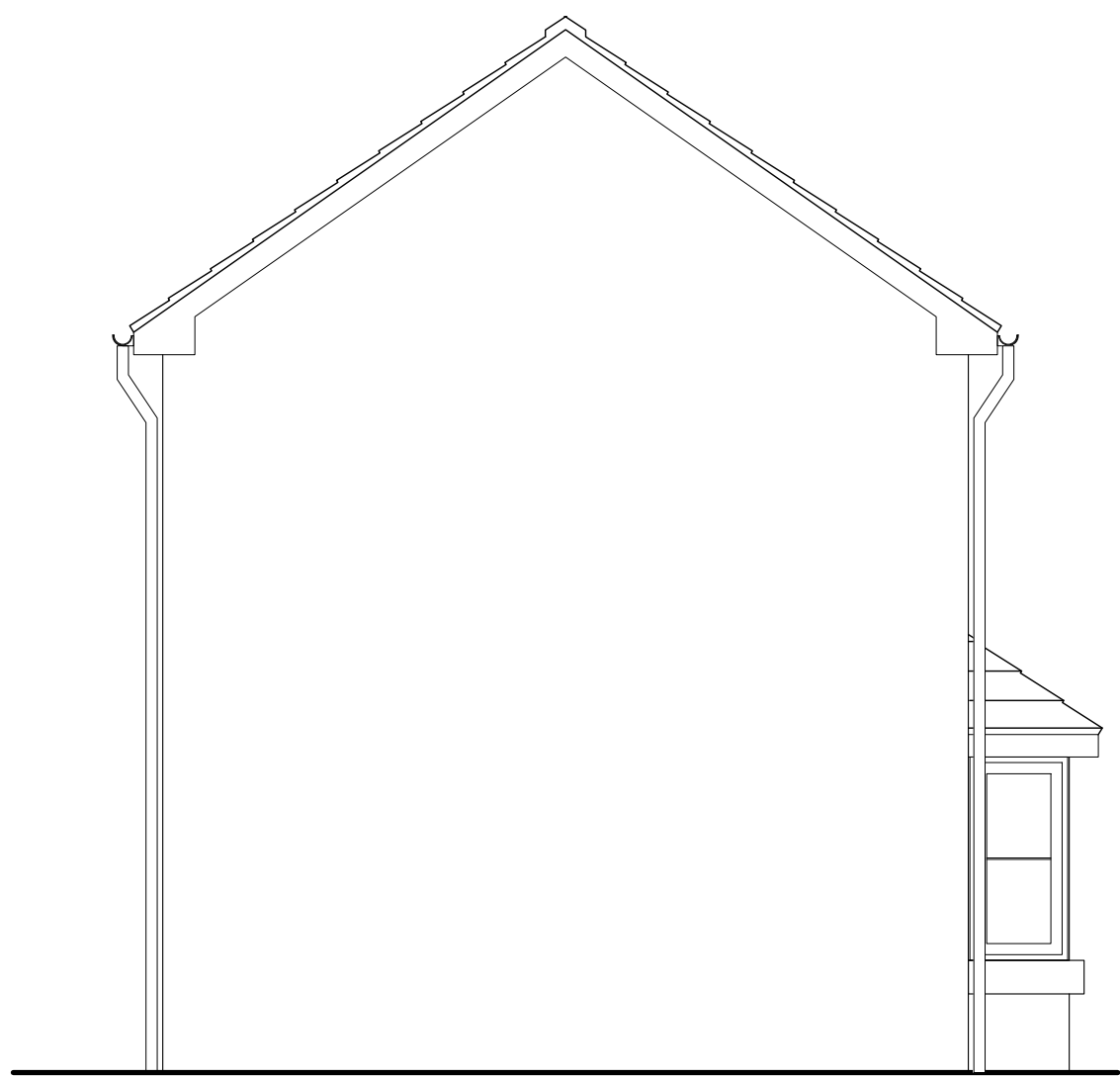
Side elevation
