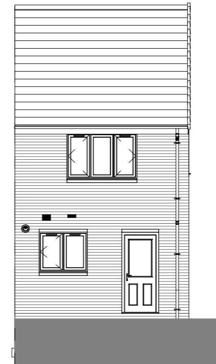
Rear Elevation.
